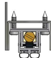
ILLUSTRATED WITH OPTIONAL 1/4" SHIM
